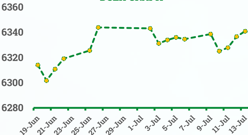
DSEX GRAPH
